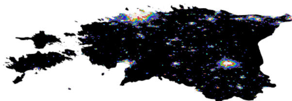
Fig. 16: Estonia's sky brightness
